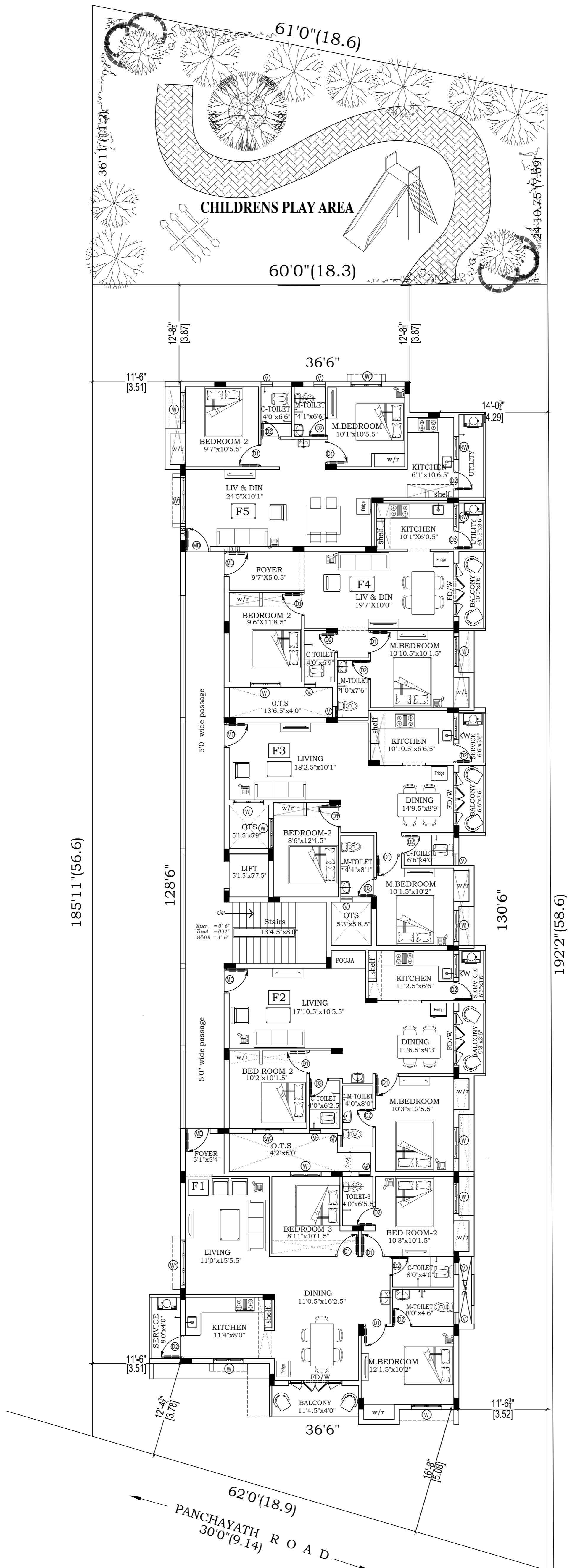
TYPICAL FLOOR PLAN
